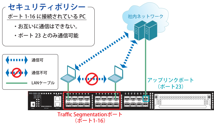
図 76-1 Traffic Segmentation (DXS-3600-32S)
