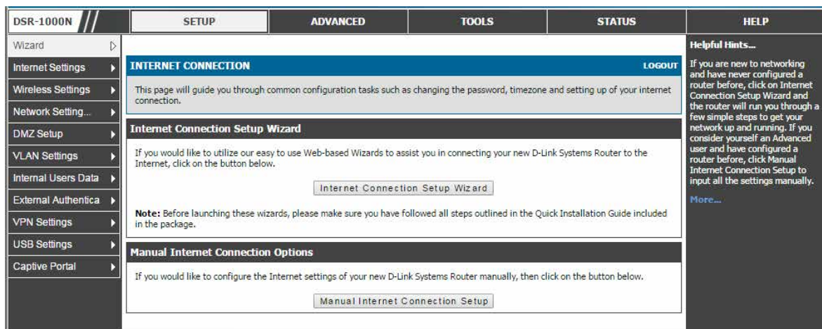
図 5-1 Internet Connection Setup Wizard
